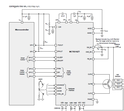
Figure 9-1. Primary Application Schematics for MCT8316ZT-Q1 (hardware variant)
