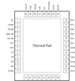
Figure 6-2. MCT8316ZT-Q1 40-Pin VQFN With Exposed Thermal Pad Top View
